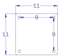
BASE PLATE FOOT PRINT
