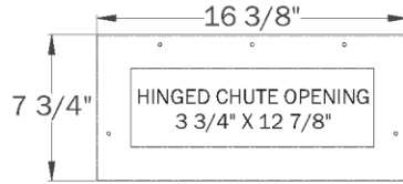
FRONT VIEW PAIRED SS FLANGE WITH PUSH PLATE
